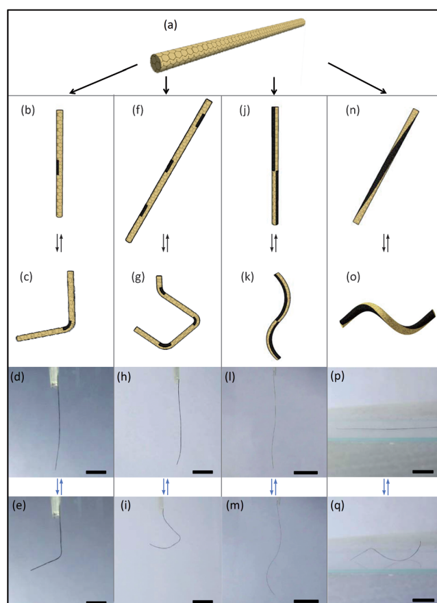
Figure 3. Schematic diagrams and photographs of different designed G/GO fibers and their reversible deformations with changes in humidity. a) The initial GO fiber. b, f, j, n) GO fibers with region-confined laser reduction. In (b) and (f) the length of reduced regions is about 1 mm, in (j) it is about 2 cm. c, g, k, o) The corresponding predefined deformations upon exposure of the fibers in (b, f, j, n) to moisture. d, h, l, p) Photographs of GO fibers corresponding to the states in (b, f, j, n). e, i, m, q) Deformations of the fibers in (d, h, l, p) at RH = 80\% . Scale bars: in (d, e, p, q): 5 mm; in (h, l, m): 1 cm.
